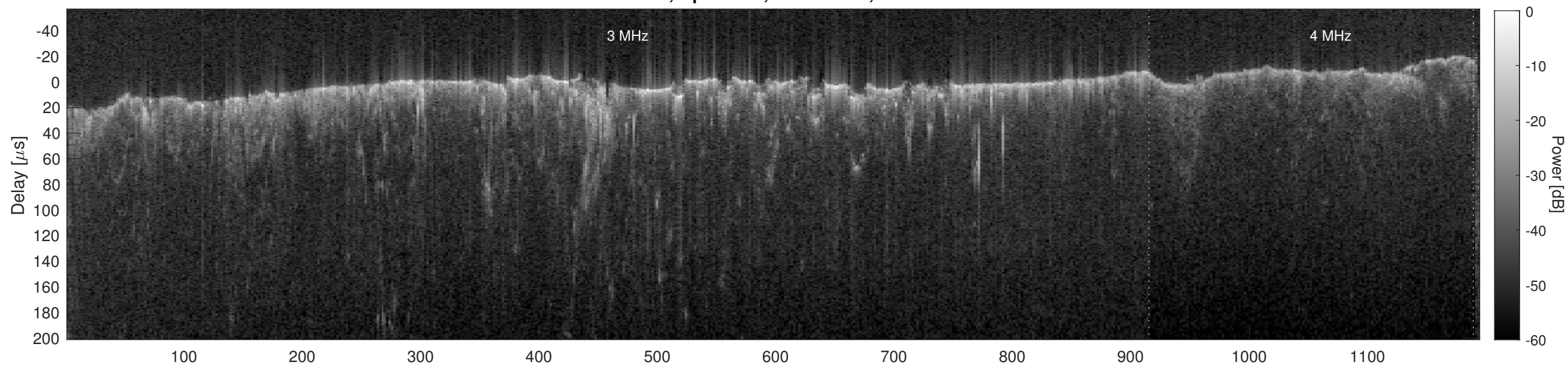
Orbit 4901, Cluttergram
