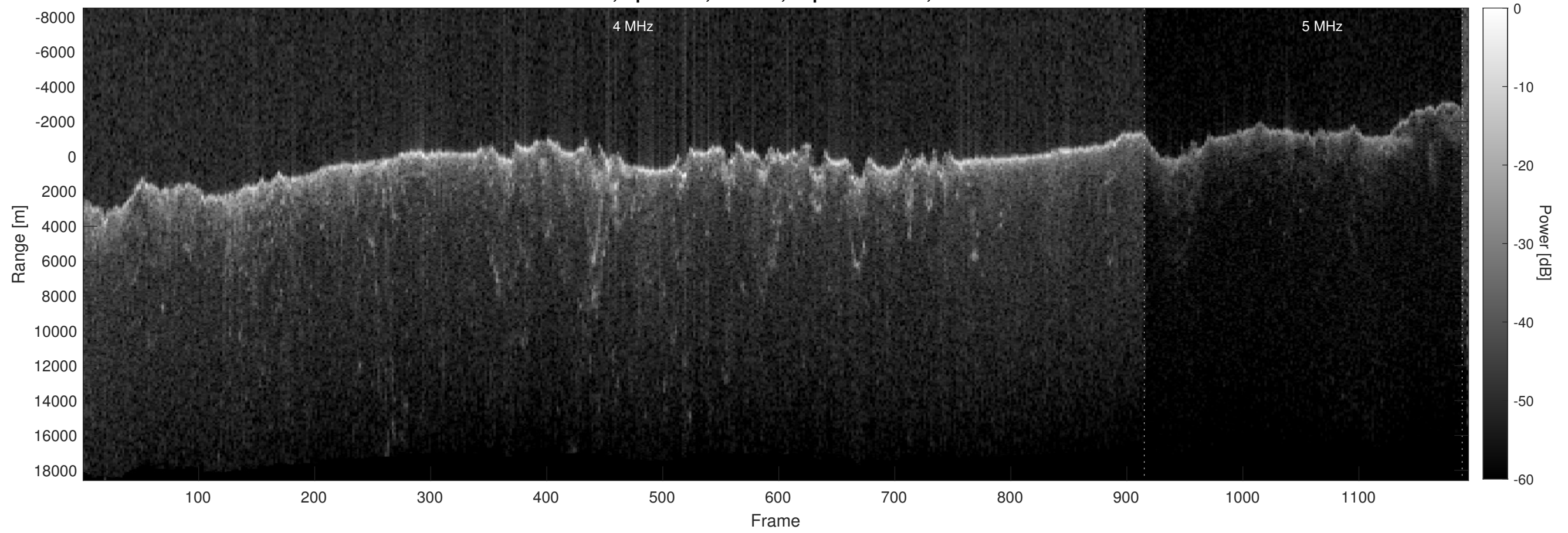
Orbit 4901, Optimized, Window, Depth-Corrected, Channel 2
