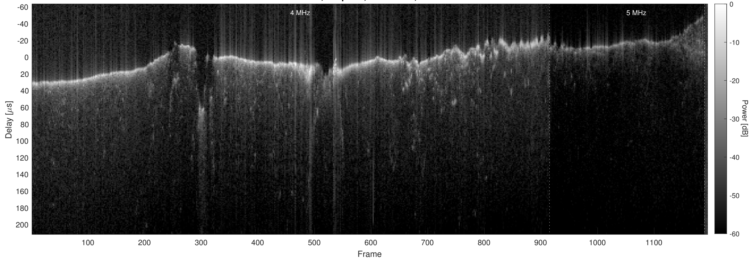
Orbit 4902, Chapman, No Window, Channel 2
