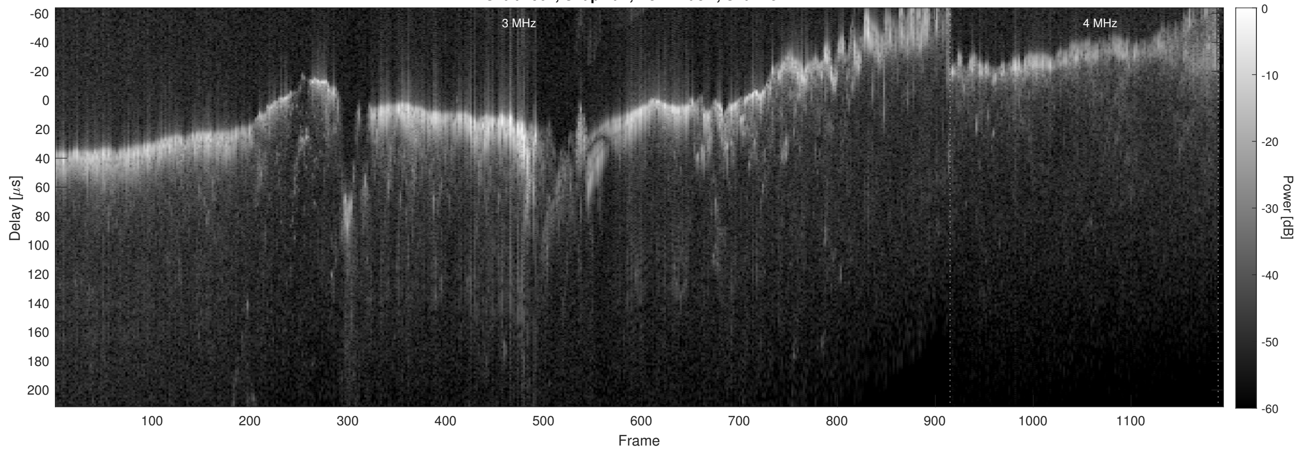
Orbit 4902, Chapman, No Window, Channel 2
