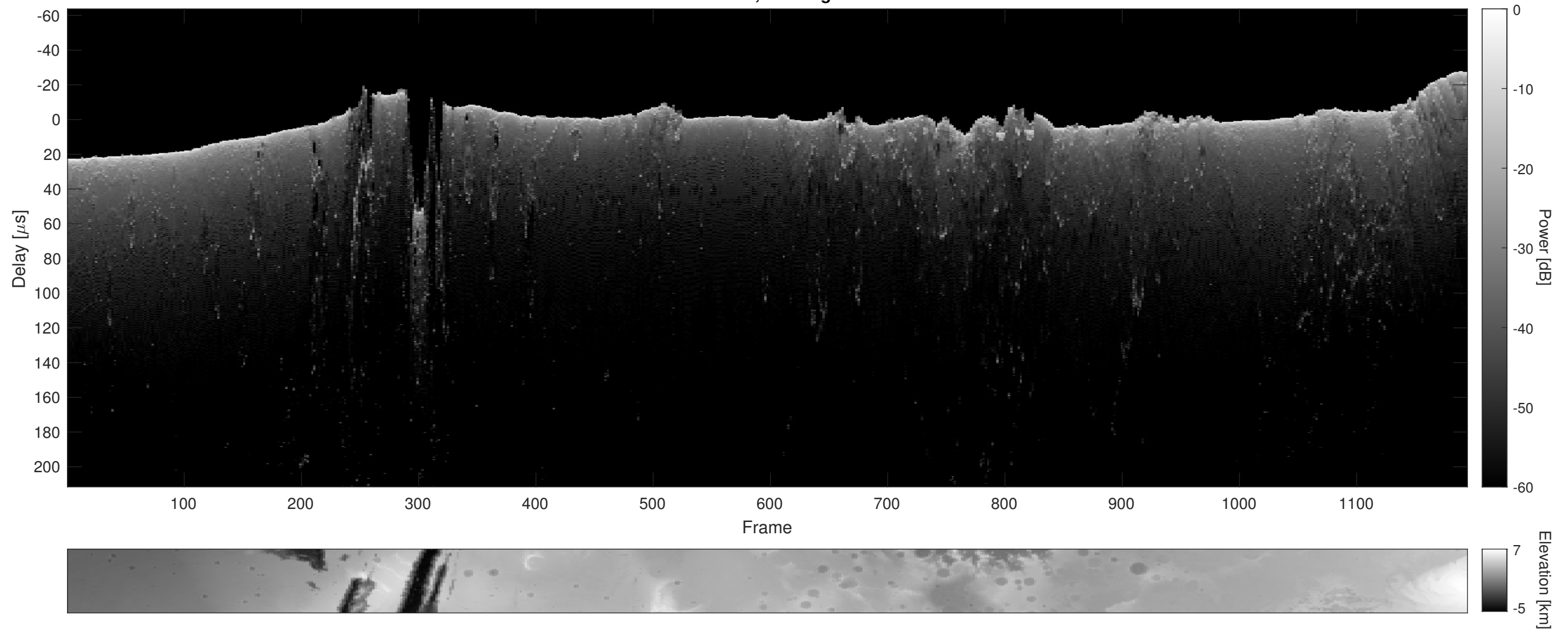
Orbit 4902, Cluttergram
