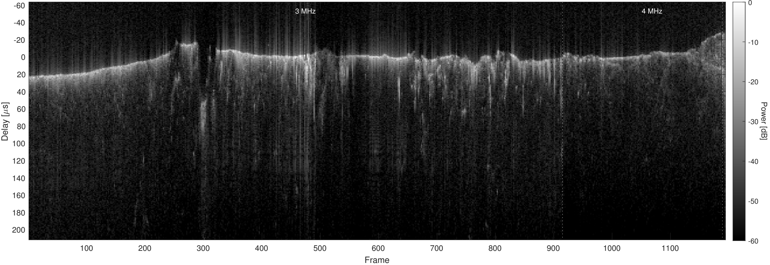
Orbit 4902, Optimized, No Window, Channel 2
