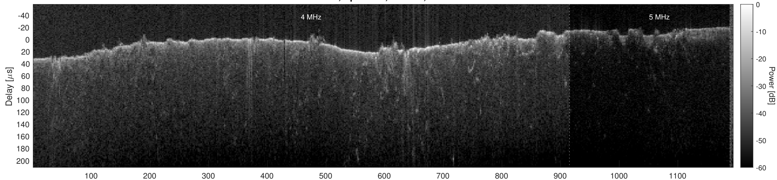
Orbit 4904, Optimized, Window, Channel 2
