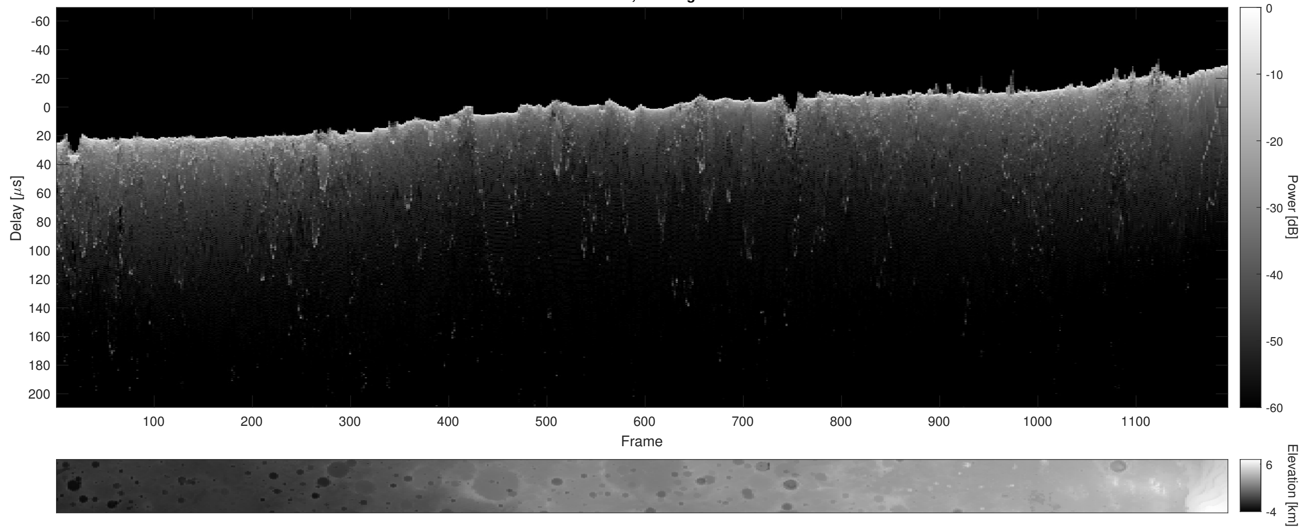
Orbit 4905, Cluttergram
