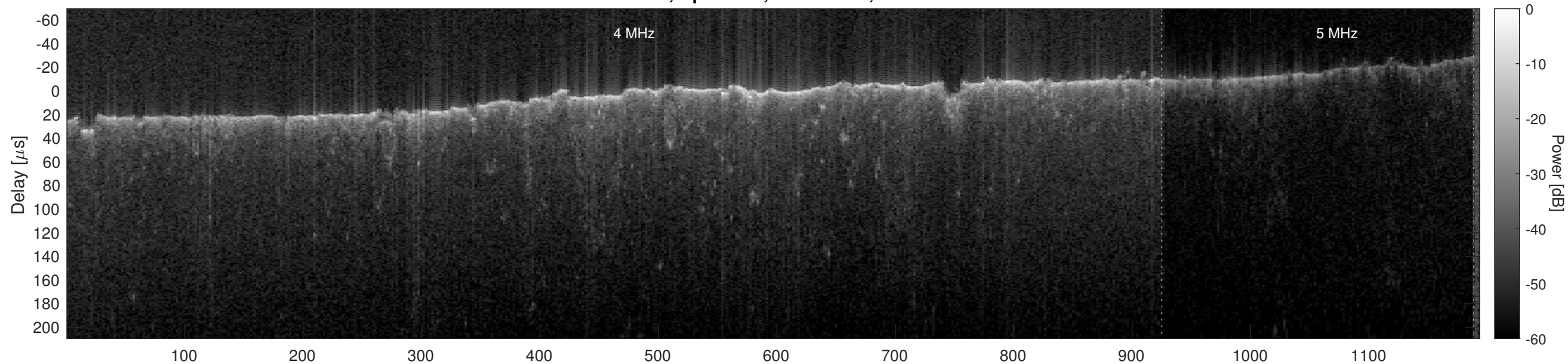
Orbit 4905, Optimized, No Window, Channel 2
