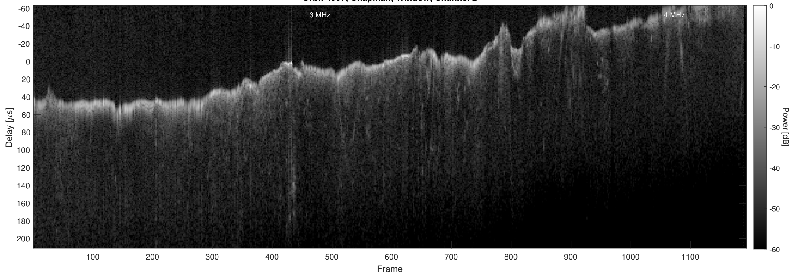
Orbit 4907, Chapman, Window, Channel 2
