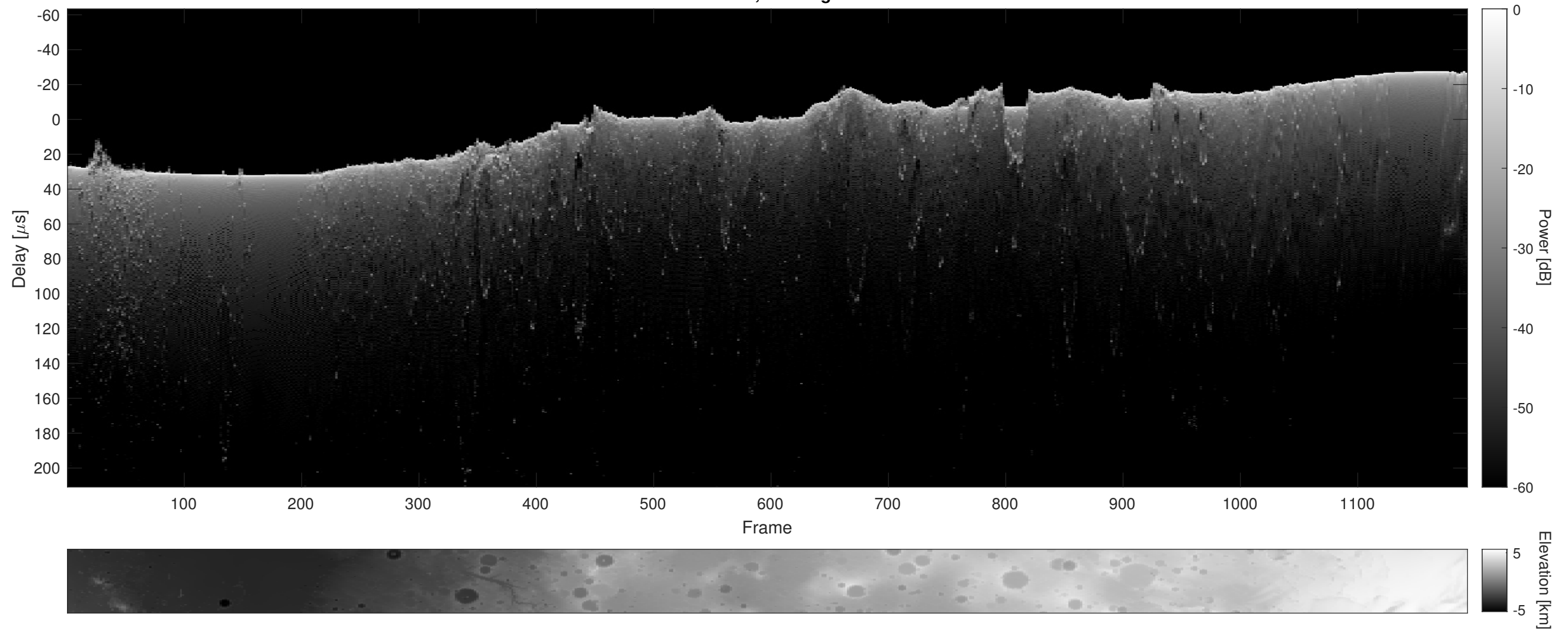
Orbit 4907, Cluttergram
