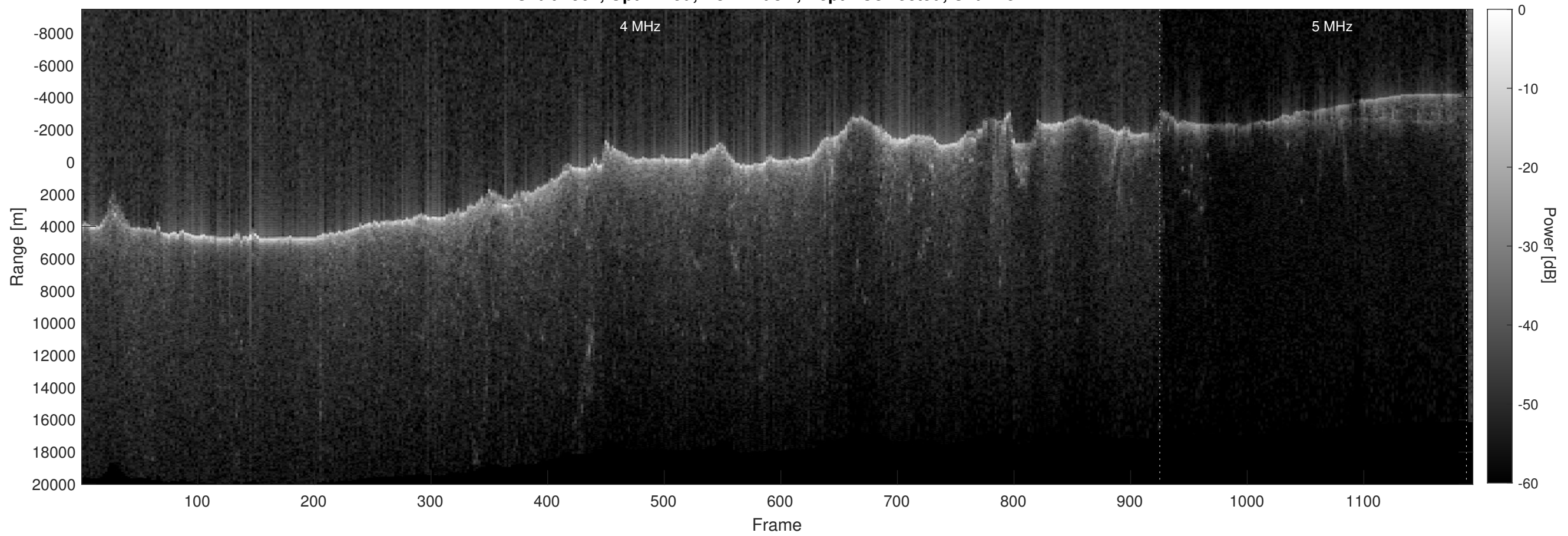
Orbit 4907, Optimized, No Window, Depth-Corrected, Channel 2
