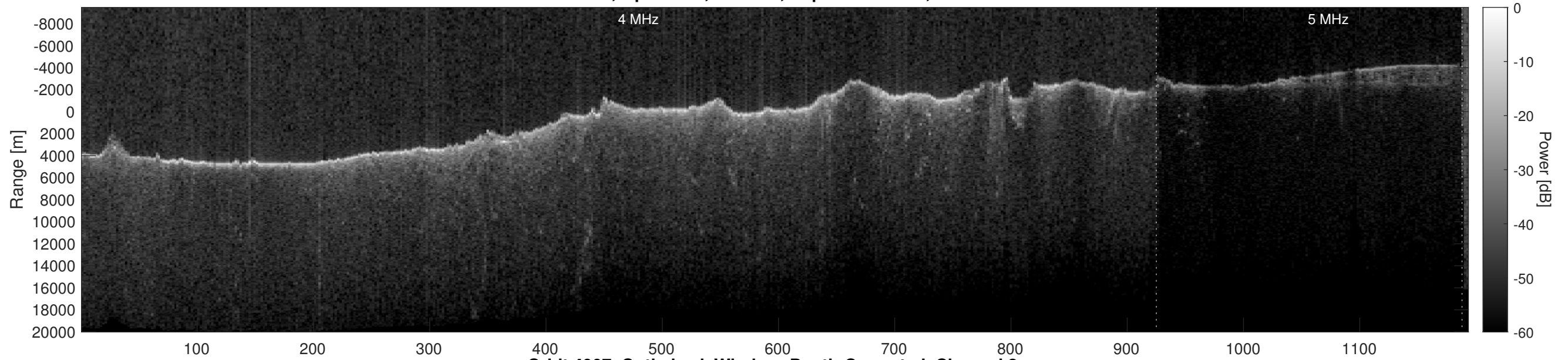
Orbit 4907, Optimized, Window, Depth-Corrected, Channel 2
