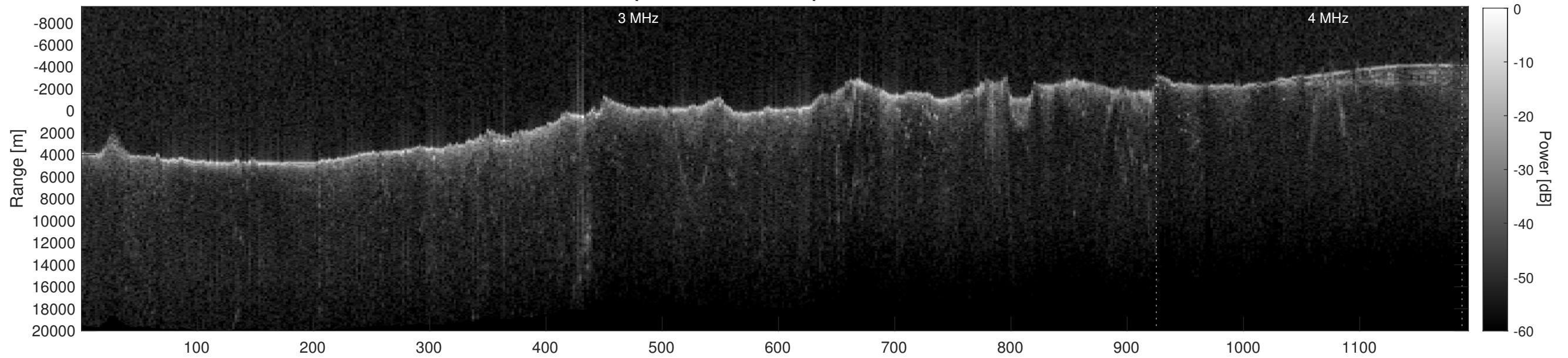
Orbit 4907, Depth-Corrected Cluttergram
