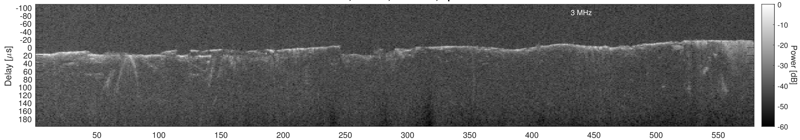
Orbit 4909, Cluttergram
