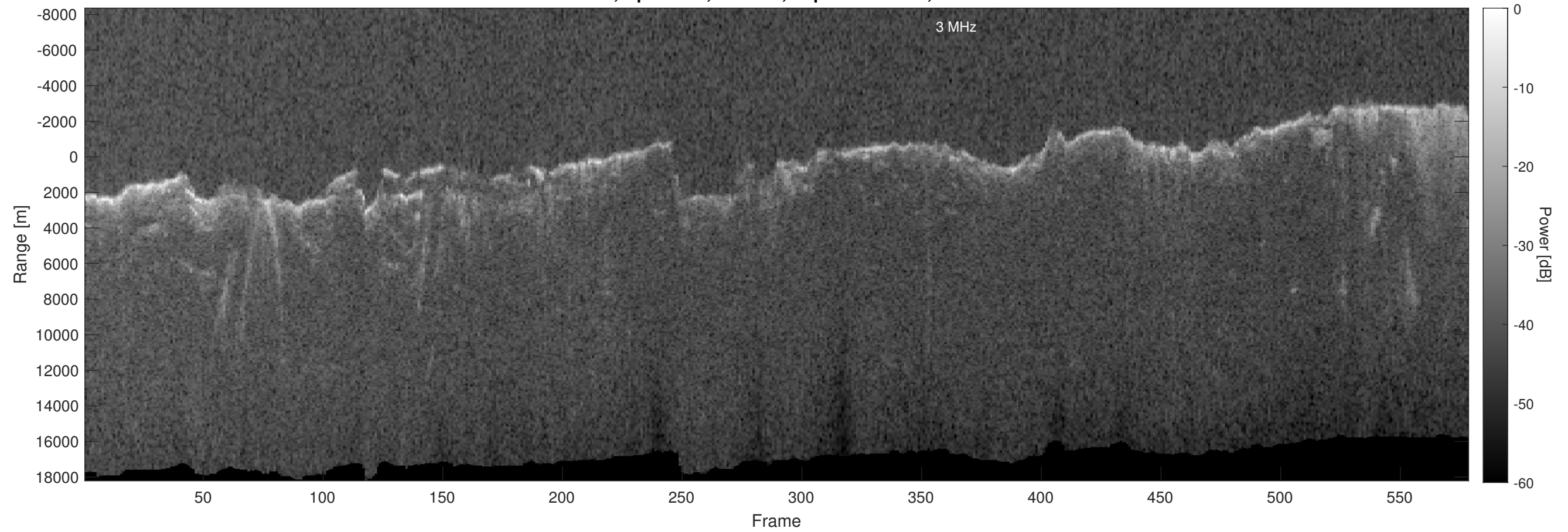
Orbit 4909, Optimized, Window, Depth-Corrected, Channel 2
