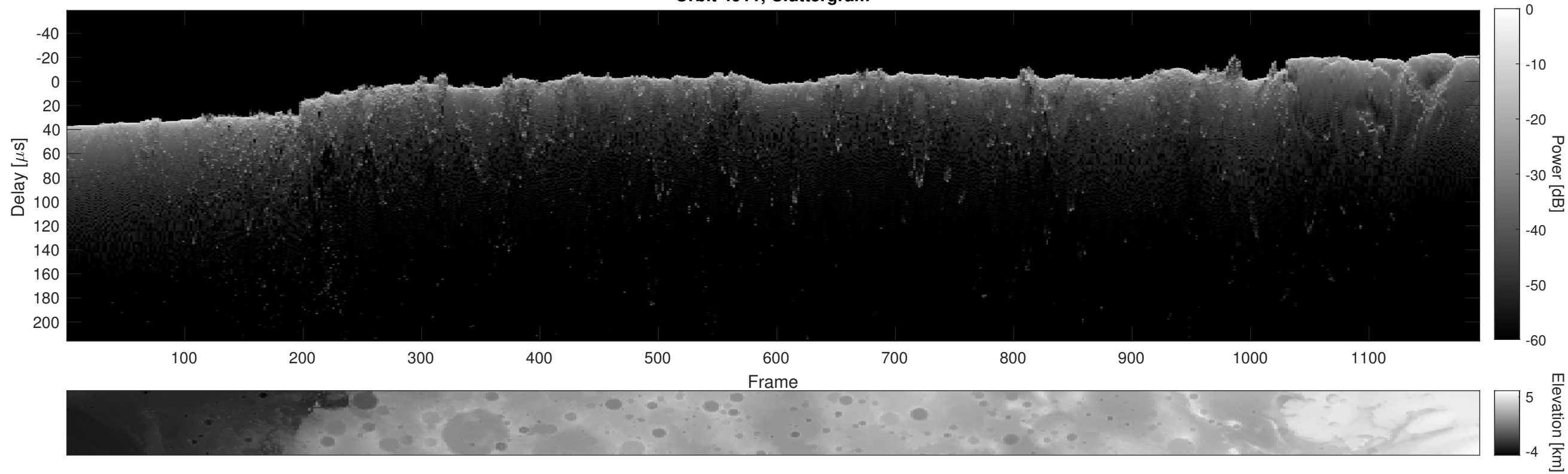
Orbit 4911, Cluttergram
