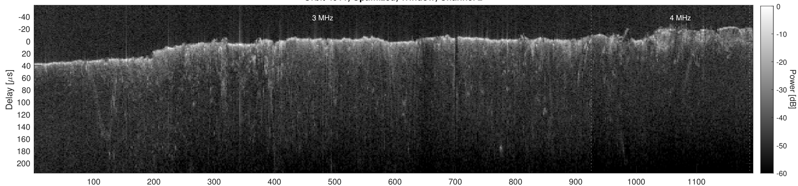
Orbit 4911, Cluttergram
