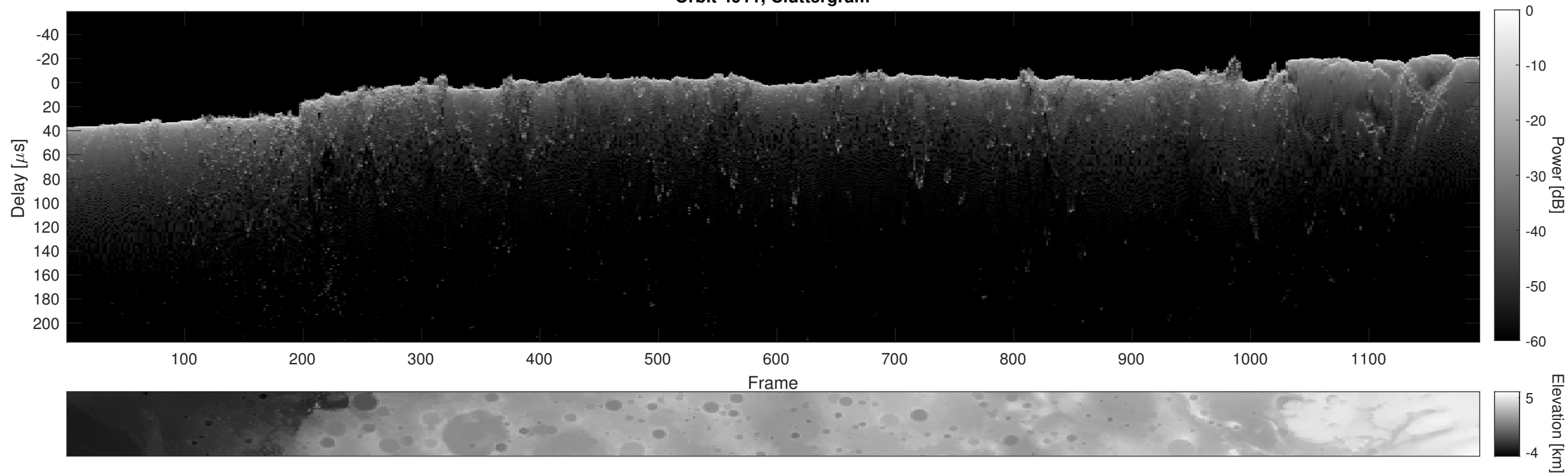
Orbit 4911, Cluttergram
