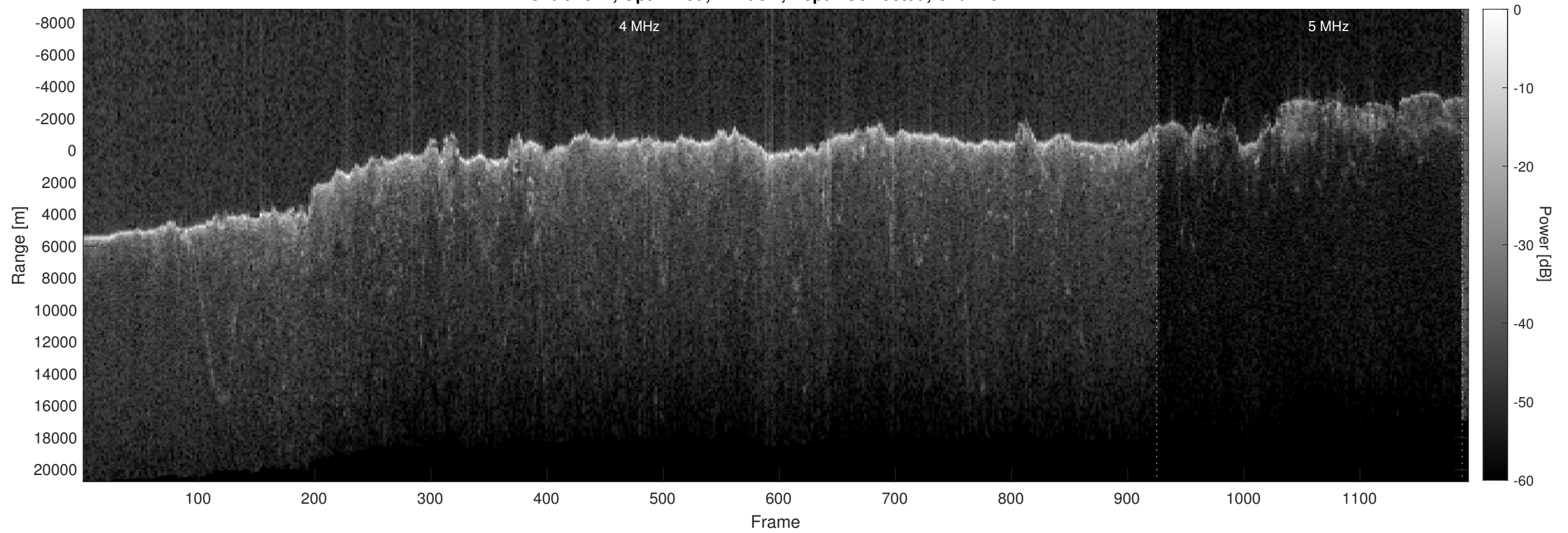
Orbit 4911, Optimized, Window, Depth-Corrected, Channel 2
