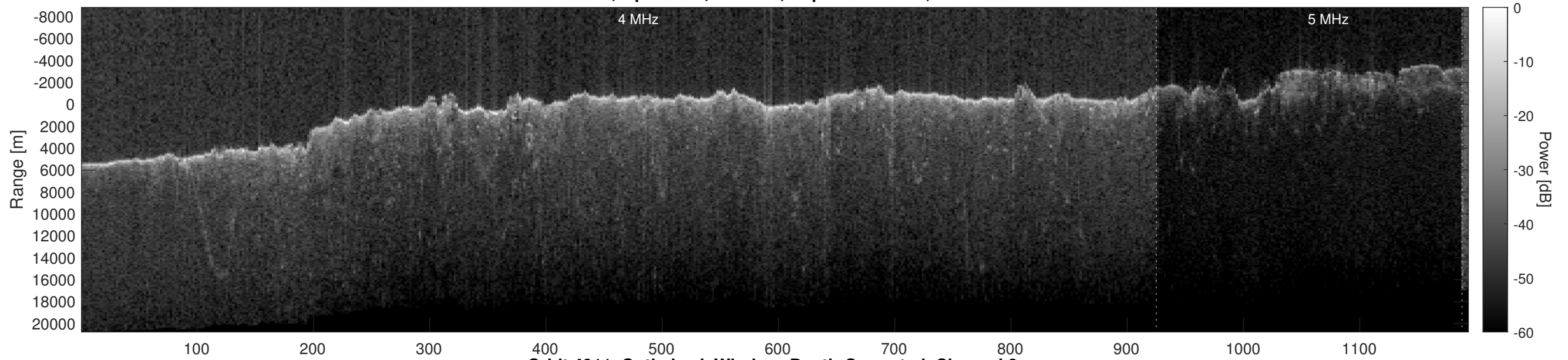
Orbit 4911, Optimized, Window, Depth-Corrected, Channel 2
