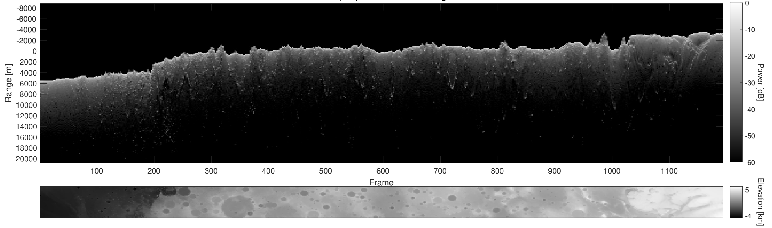
Orbit 4911, Depth-Corrected Cluttergram
