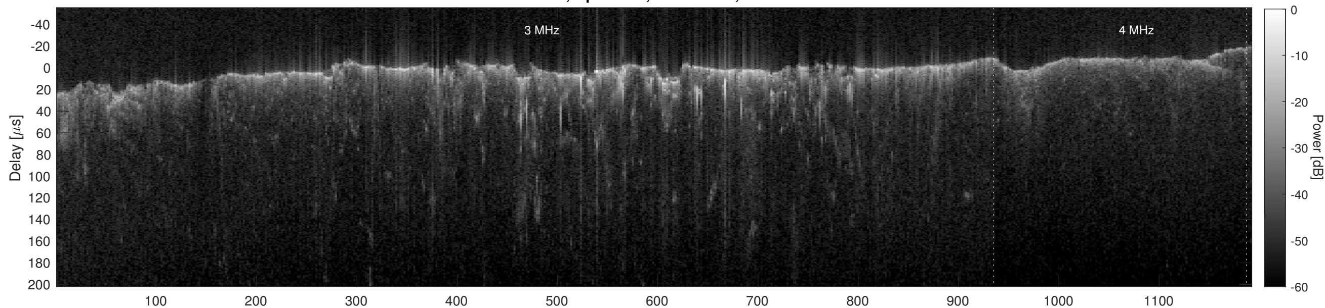
Orbit 4912, Cluttergram
