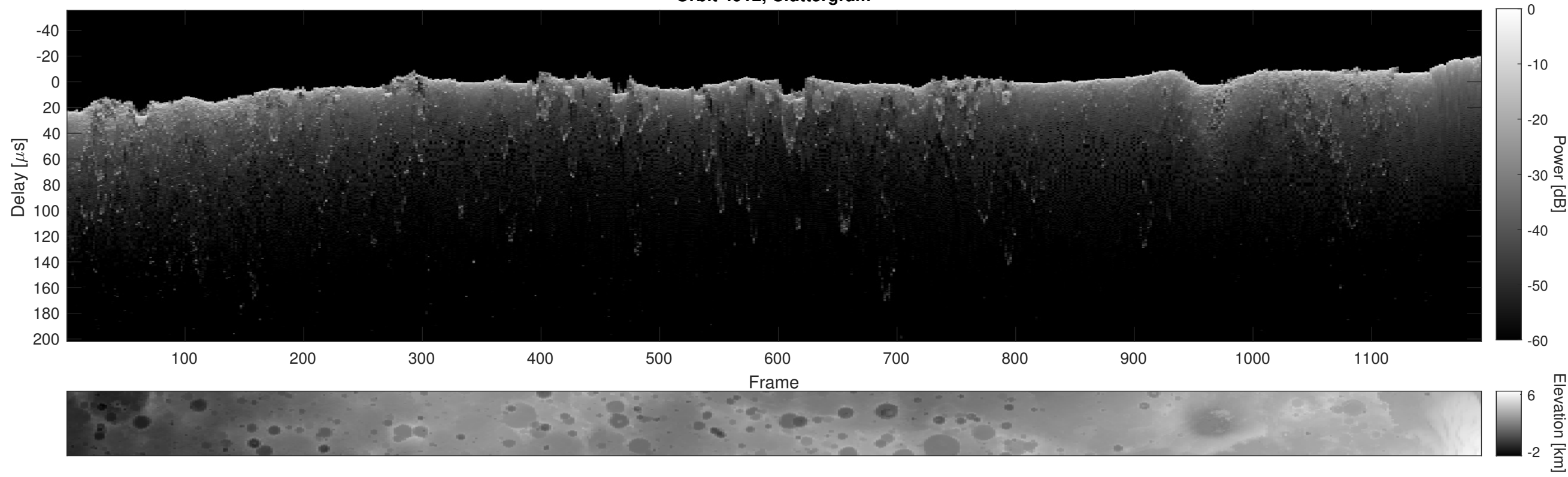
Orbit 4912, Cluttergram
