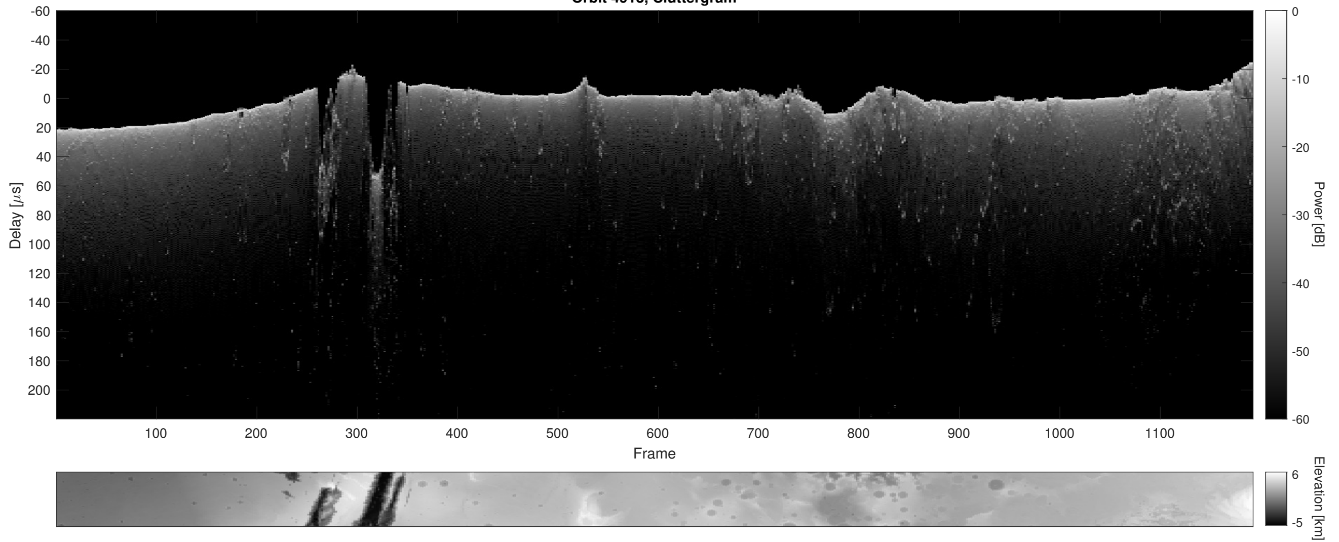
Orbit 4913, Cluttergram
