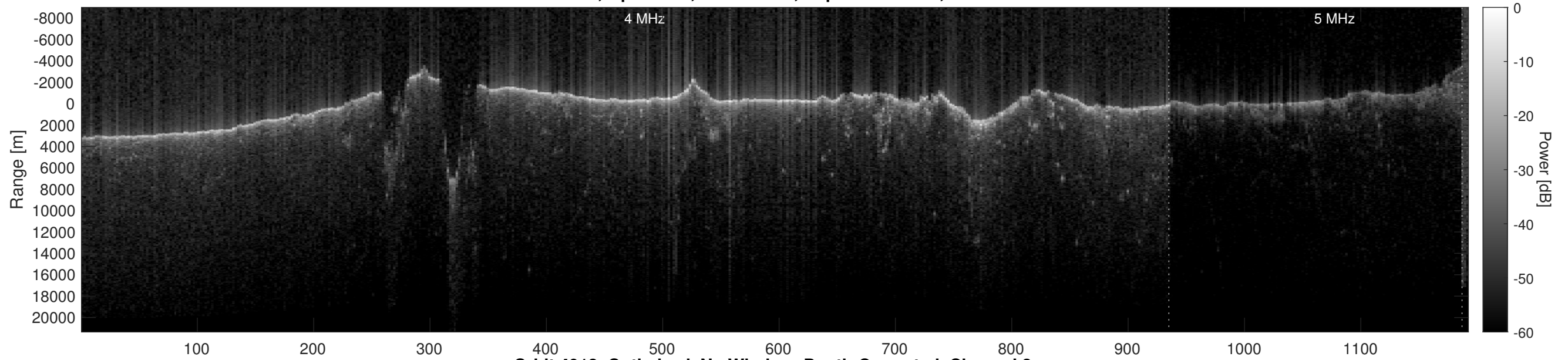
Orbit 4913, Optimized, No Window, Depth-Corrected, Channel 2
