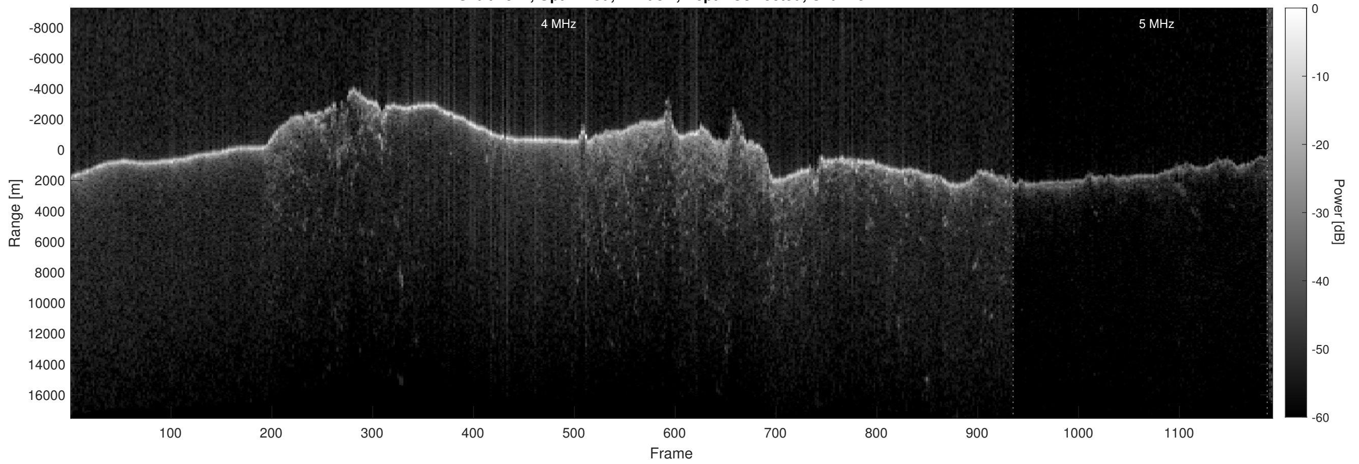
Orbit 4917, Optimized, Window, Depth-Corrected, Channel 2
