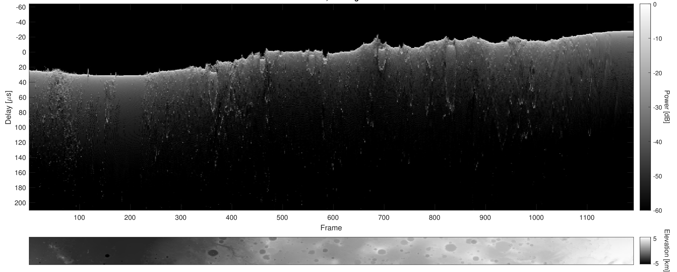
Orbit 4918, Cluttergram
