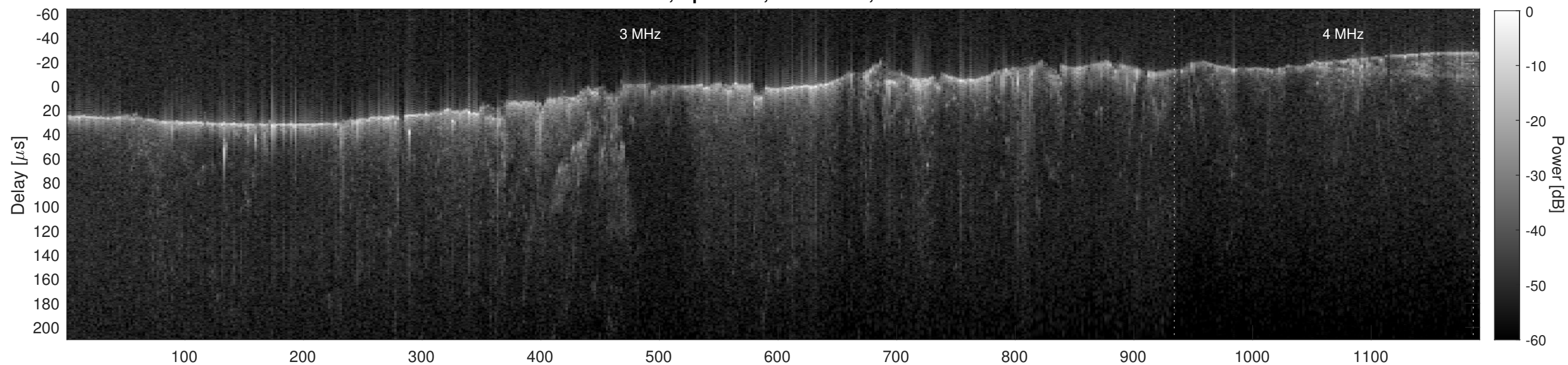
Orbit 4918, Cluttergram
