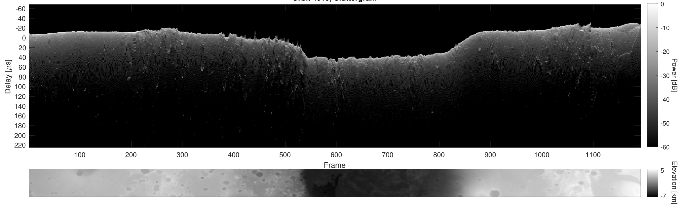
Orbit 4919, Cluttergram
