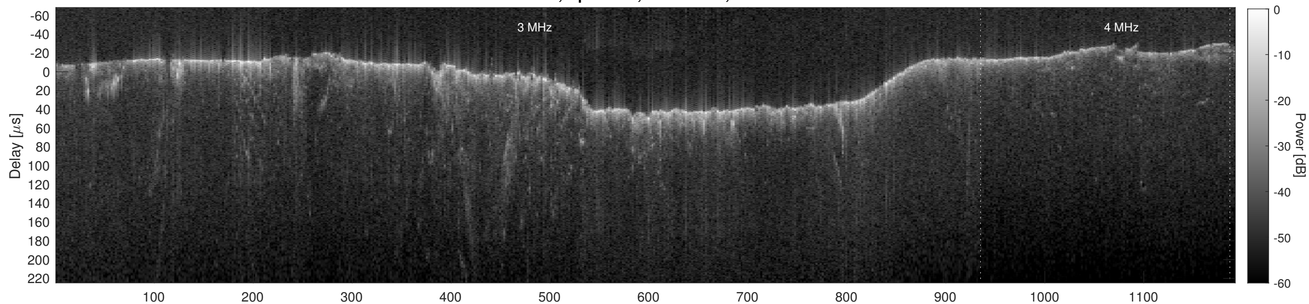
Orbit 4919, Cluttergram
