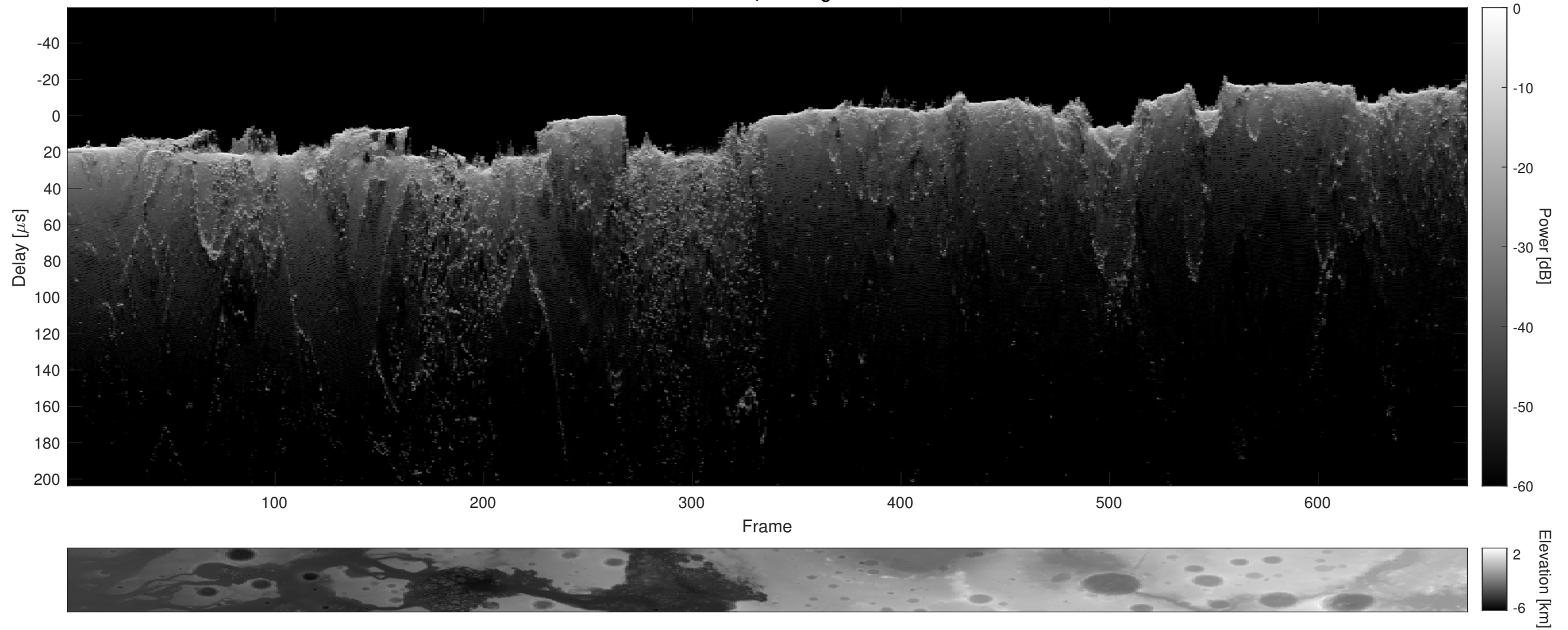
Orbit 4920, Cluttergram
