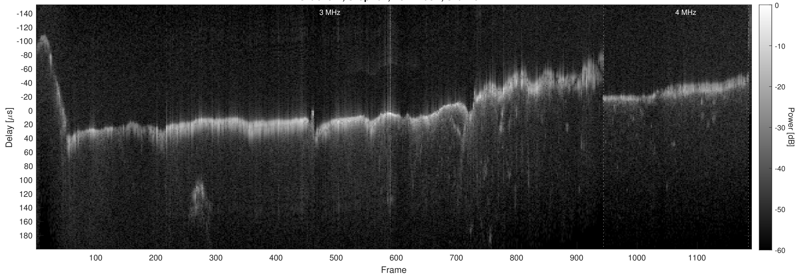
Orbit 4921, Chapman, No Window, Channel 2
