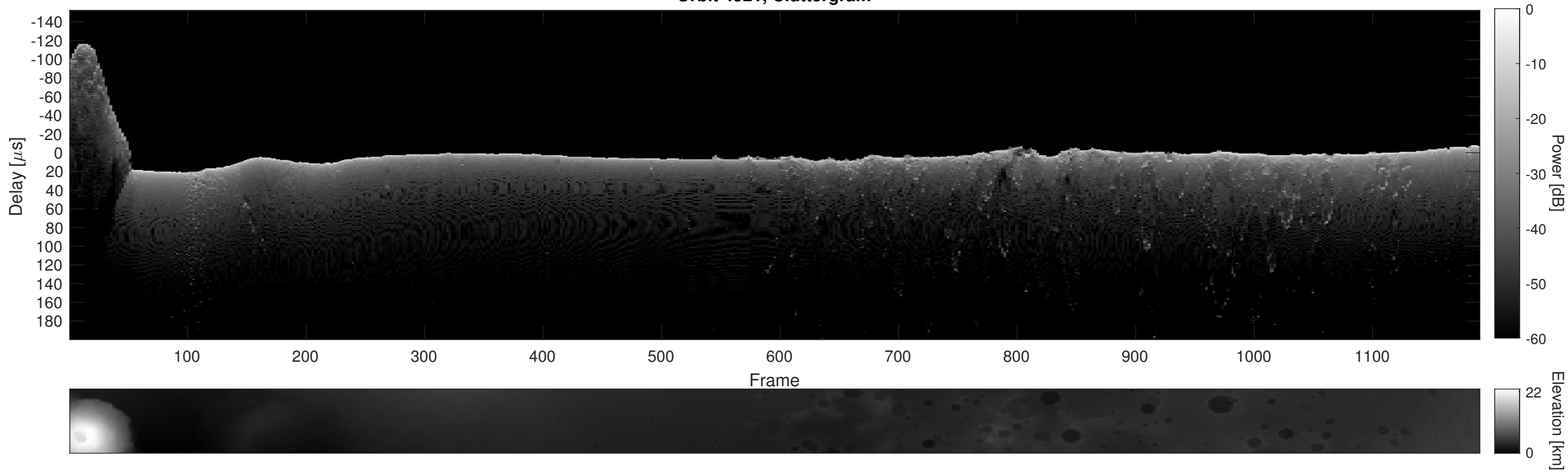
Orbit 4921, Cluttergram
