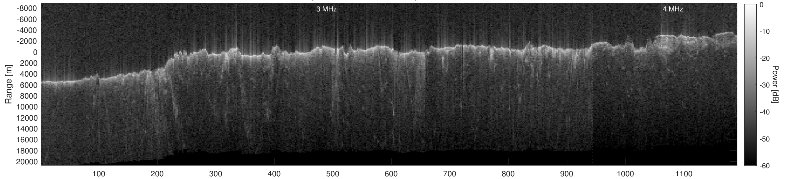
Orbit 4922, Depth-Corrected Cluttergram
