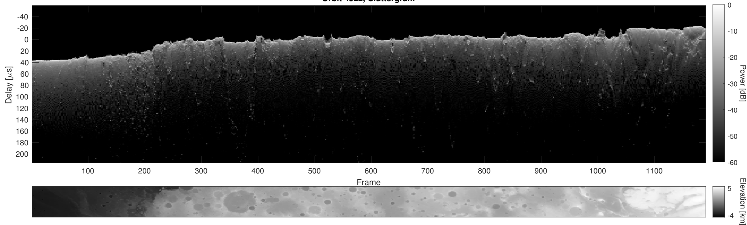
Orbit 4922, Cluttergram
