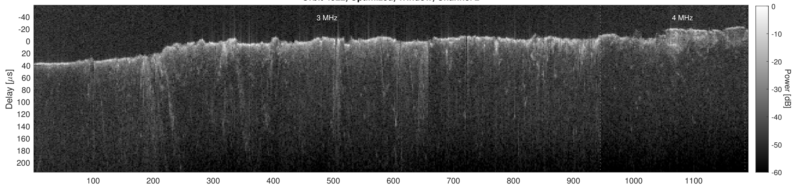
Orbit 4922, Cluttergram
