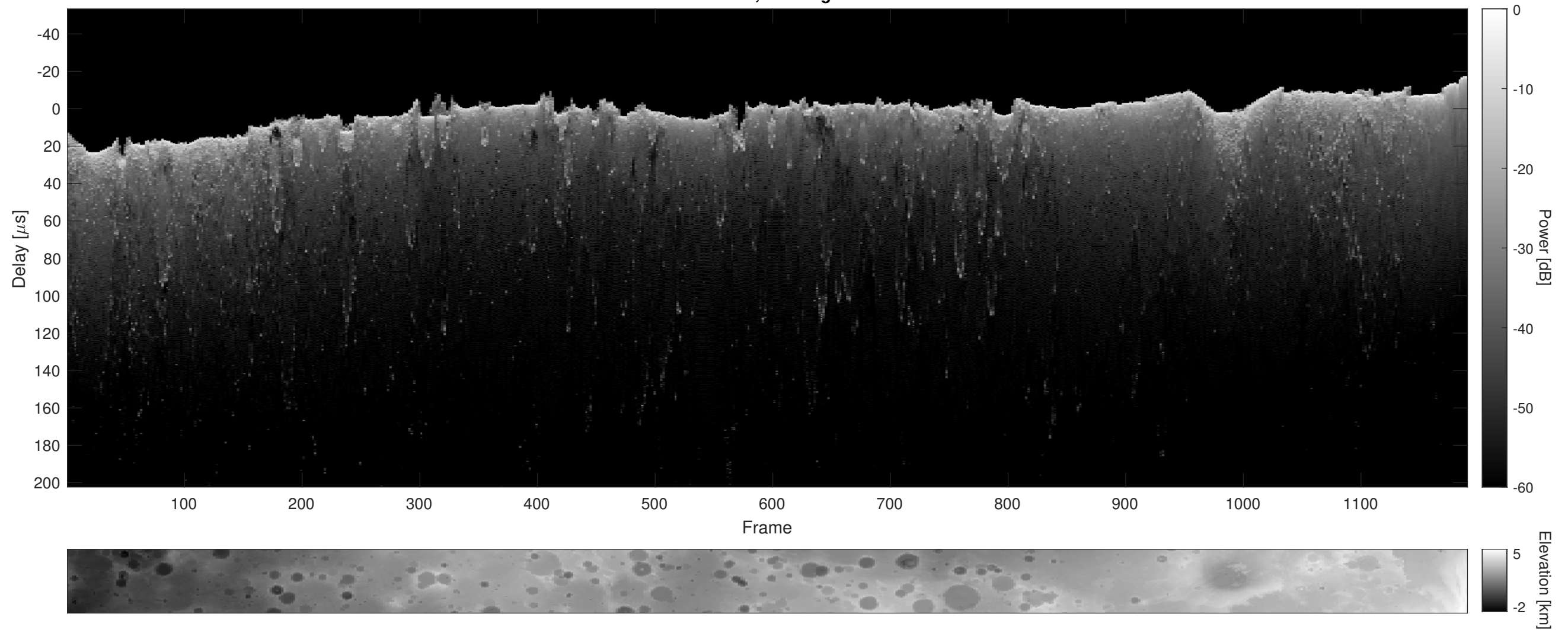
Orbit 4923, Cluttergram
