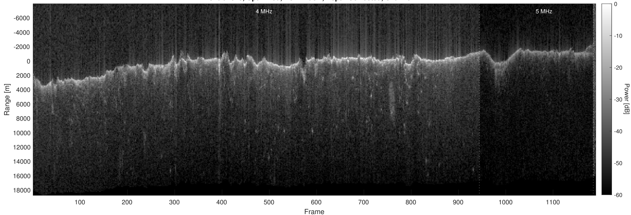
Orbit 4923, Optimized, No Window, Depth-Corrected, Channel 2
