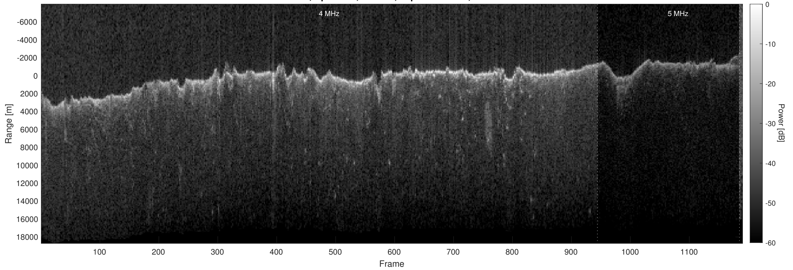
Orbit 4923, Optimized, Window, Depth-Corrected, Channel 2
