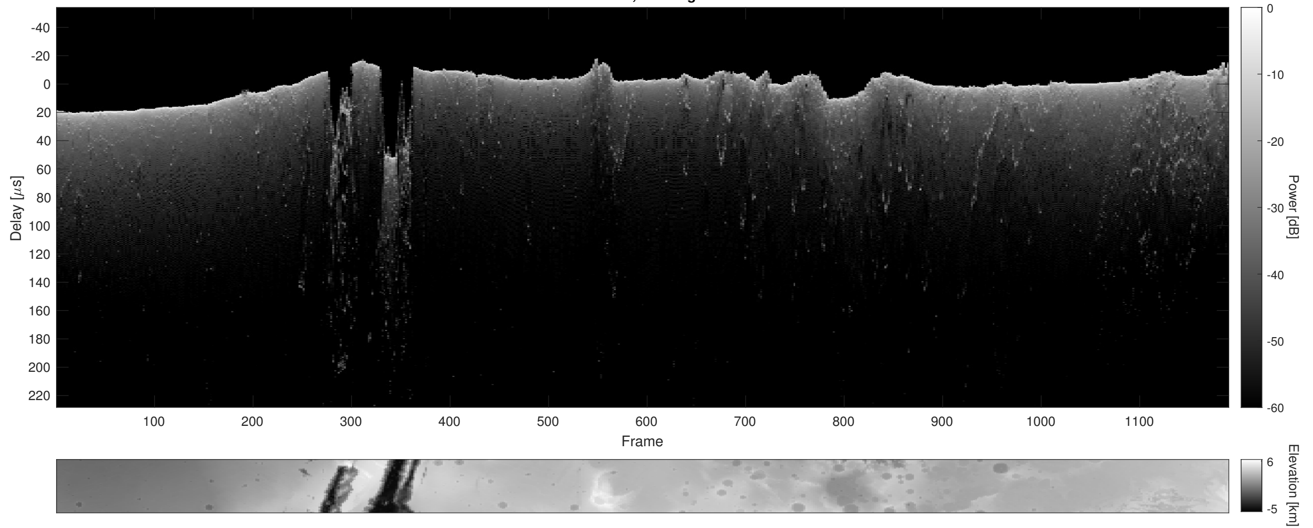
Orbit 4924, Cluttergram
