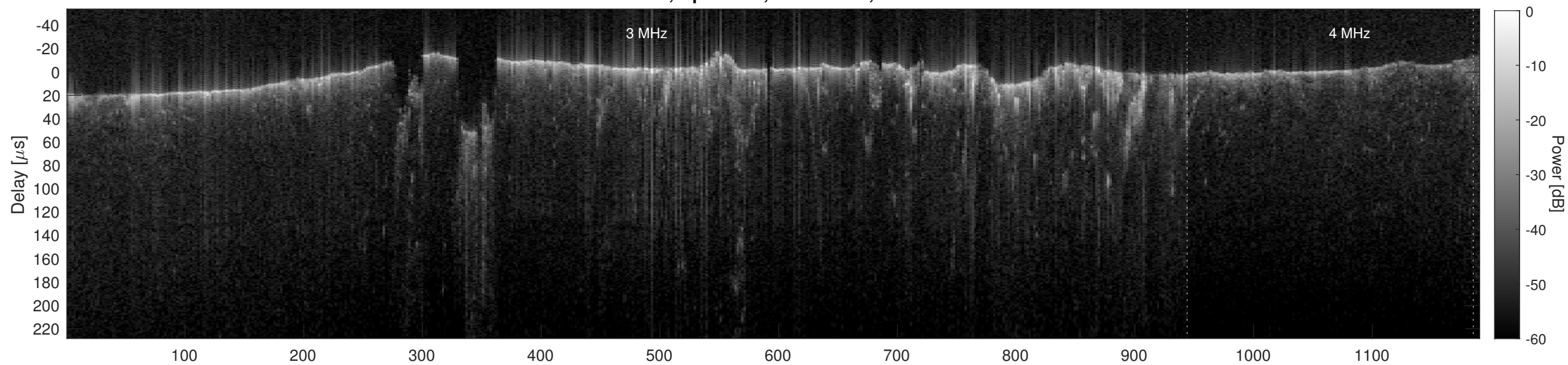
Orbit 4924, Cluttergram
