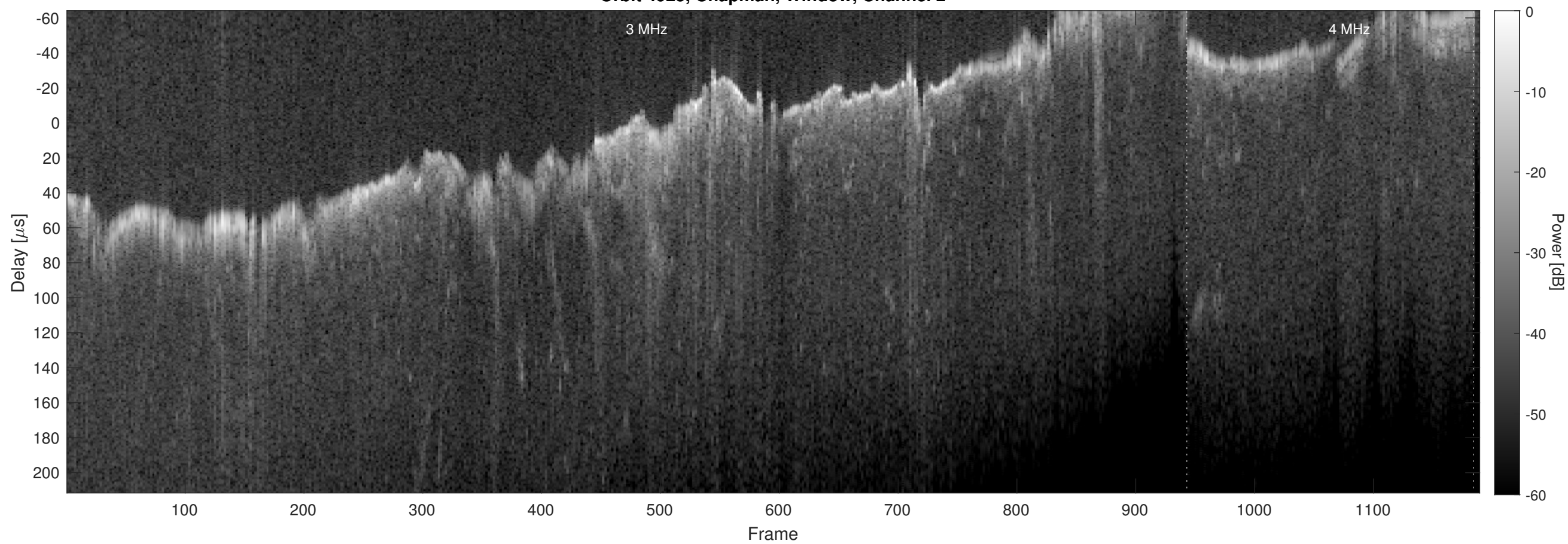
Orbit 4925, Chapman, Window, Channel 2
