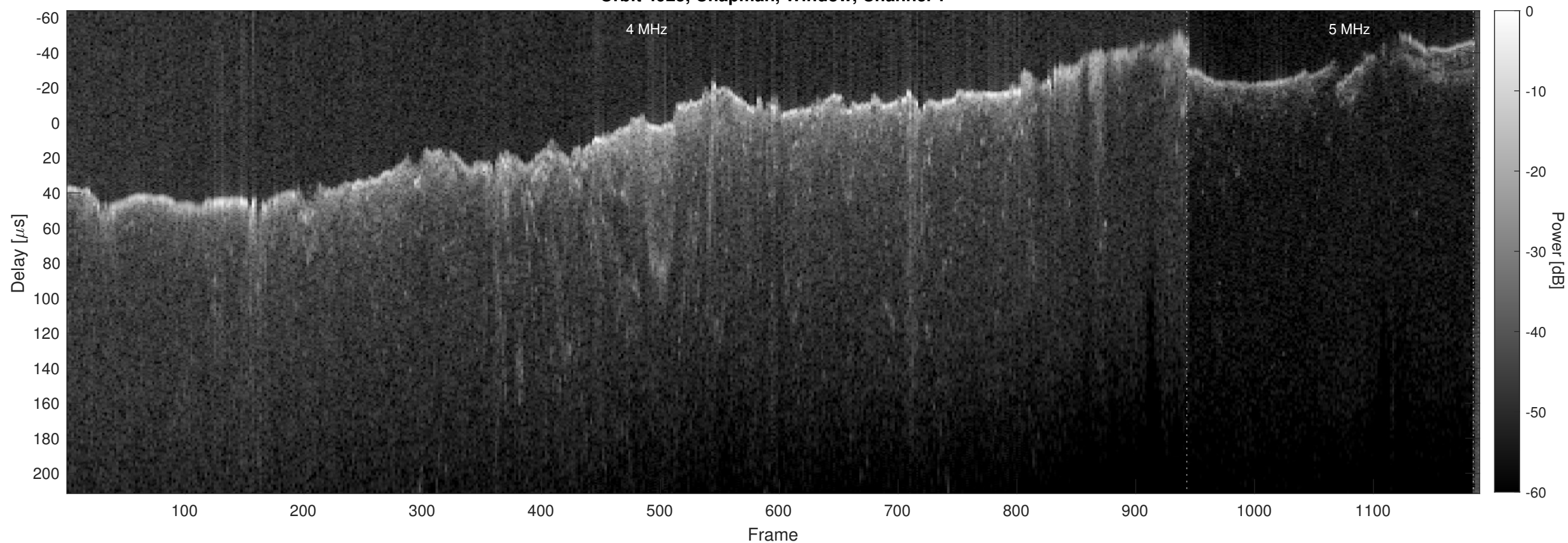
Orbit 4925, Chapman, Window, Channel 2
