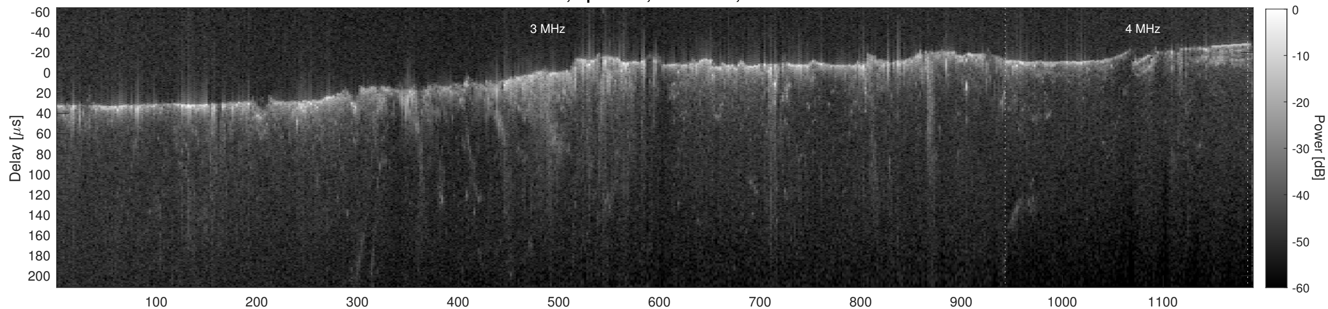
Orbit 4925, Cluttergram
