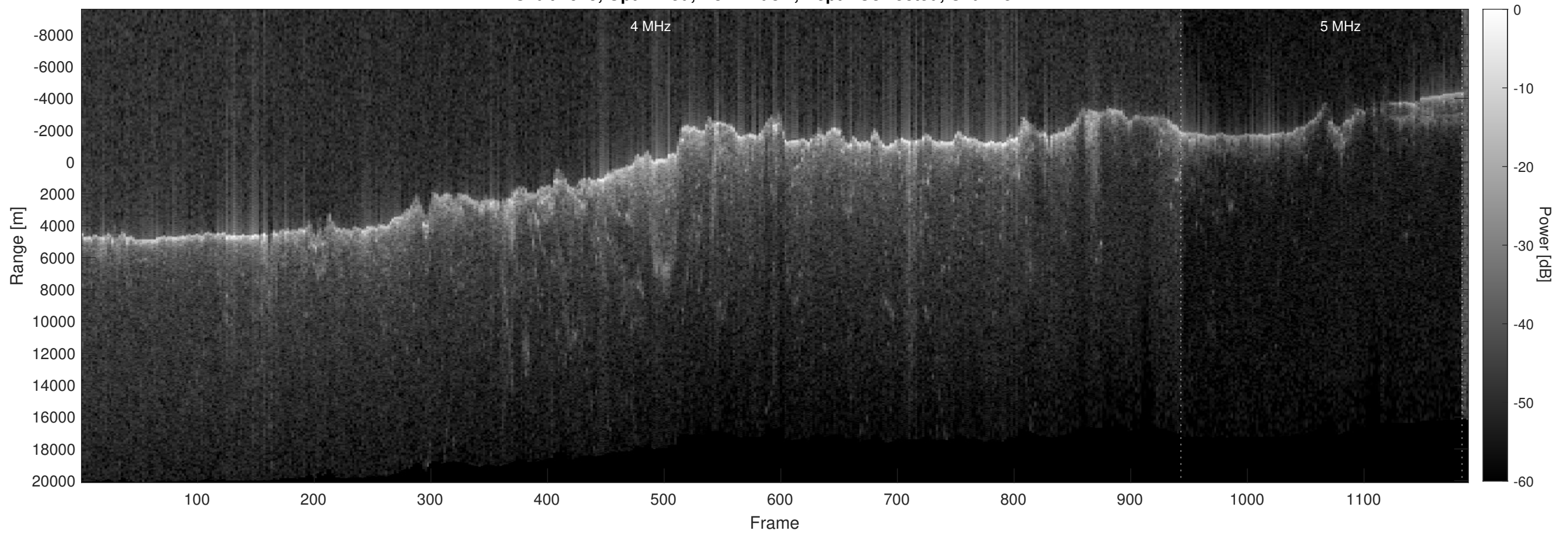
Orbit 4925, Optimized, No Window, Depth-Corrected, Channel 2
