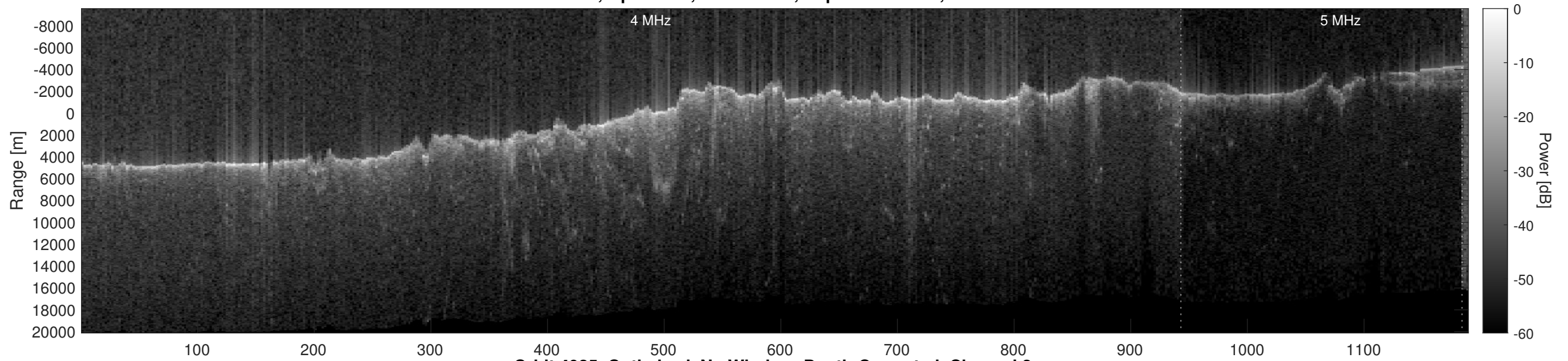
Orbit 4925, Optimized, No Window, Depth-Corrected, Channel 2
