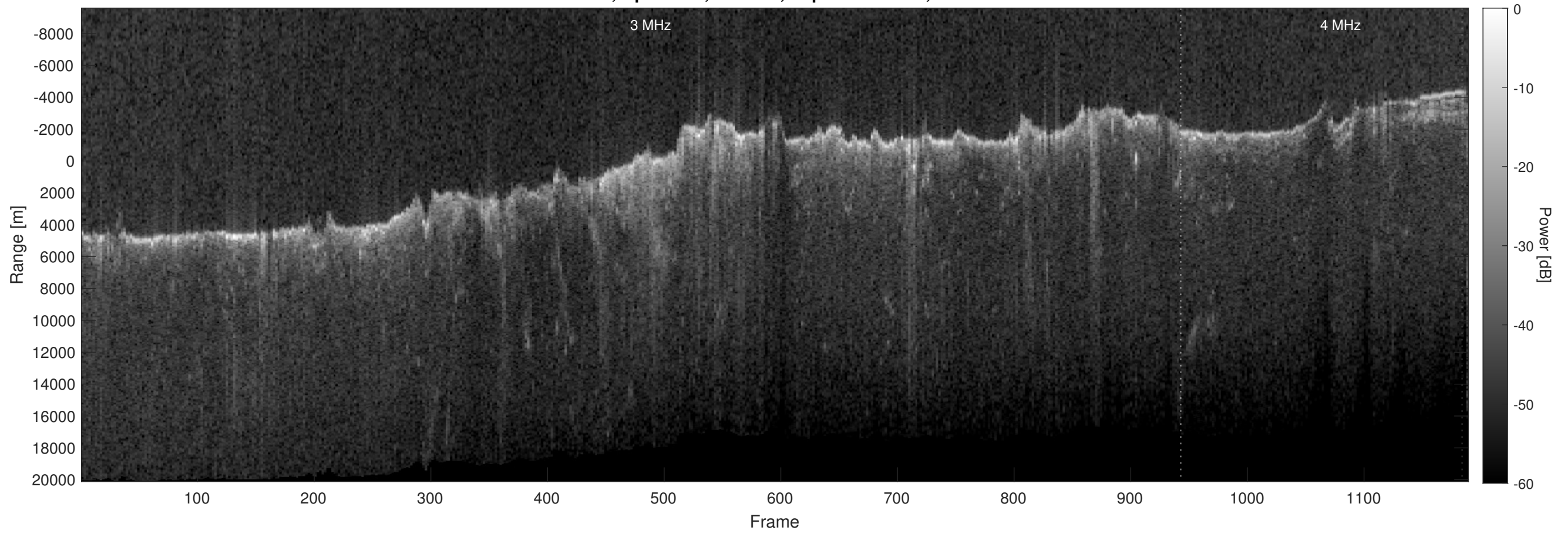
Orbit 4925, Optimized, Window, Depth-Corrected, Channel 2
