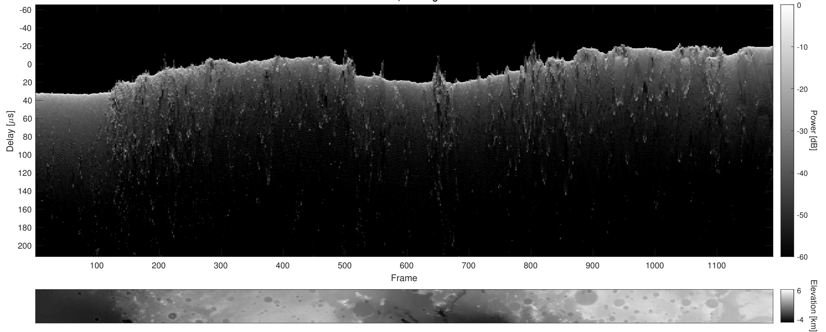
Orbit 4926, Cluttergram
