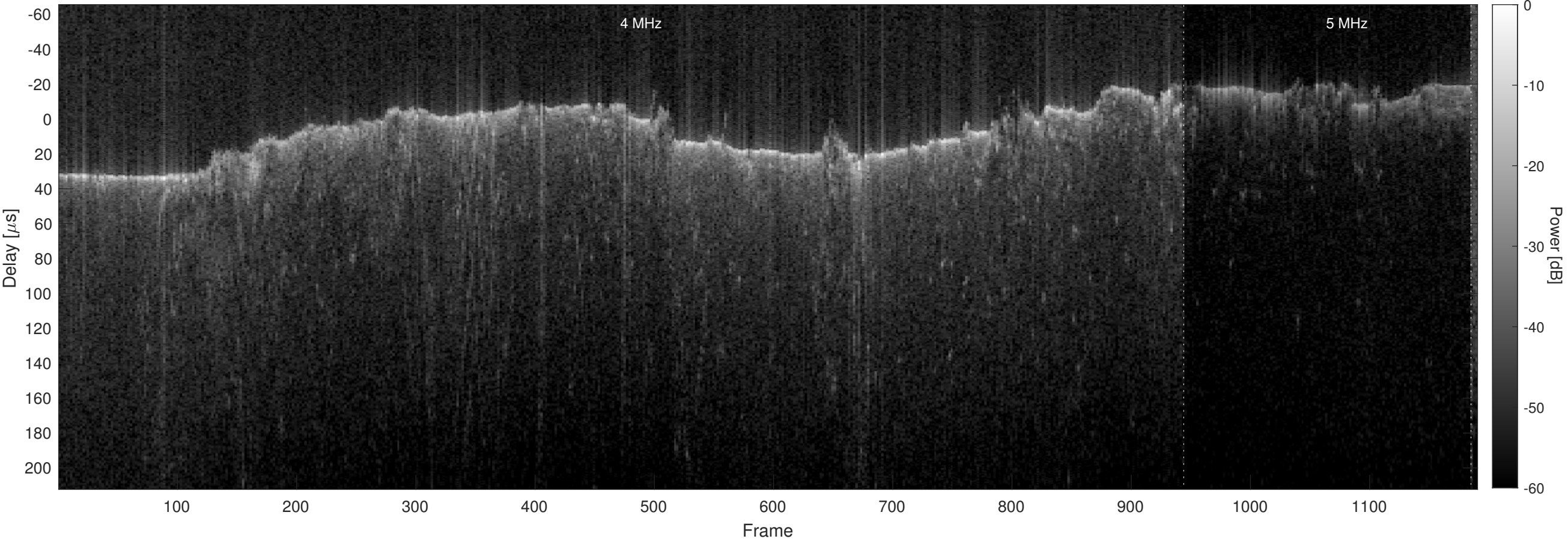
Orbit 4926, Optimized, No Window, Channel 2
