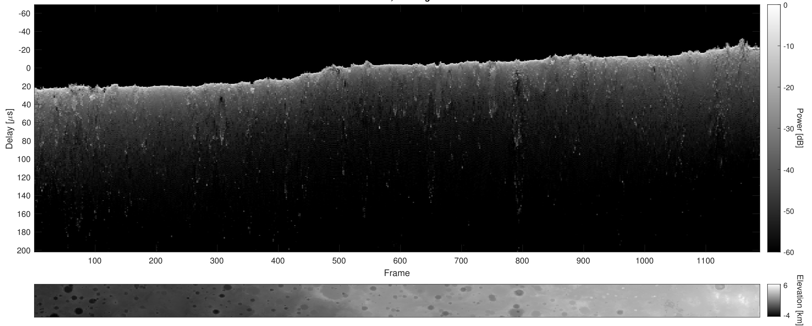
Orbit 4927, Cluttergram
