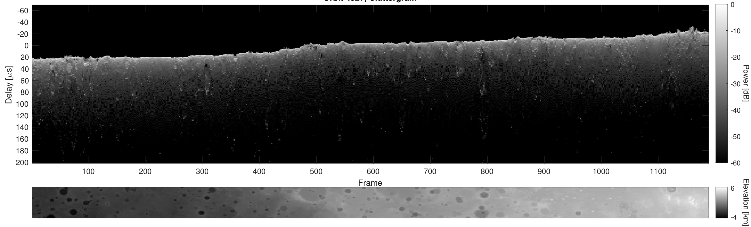
Orbit 4927, Cluttergram
