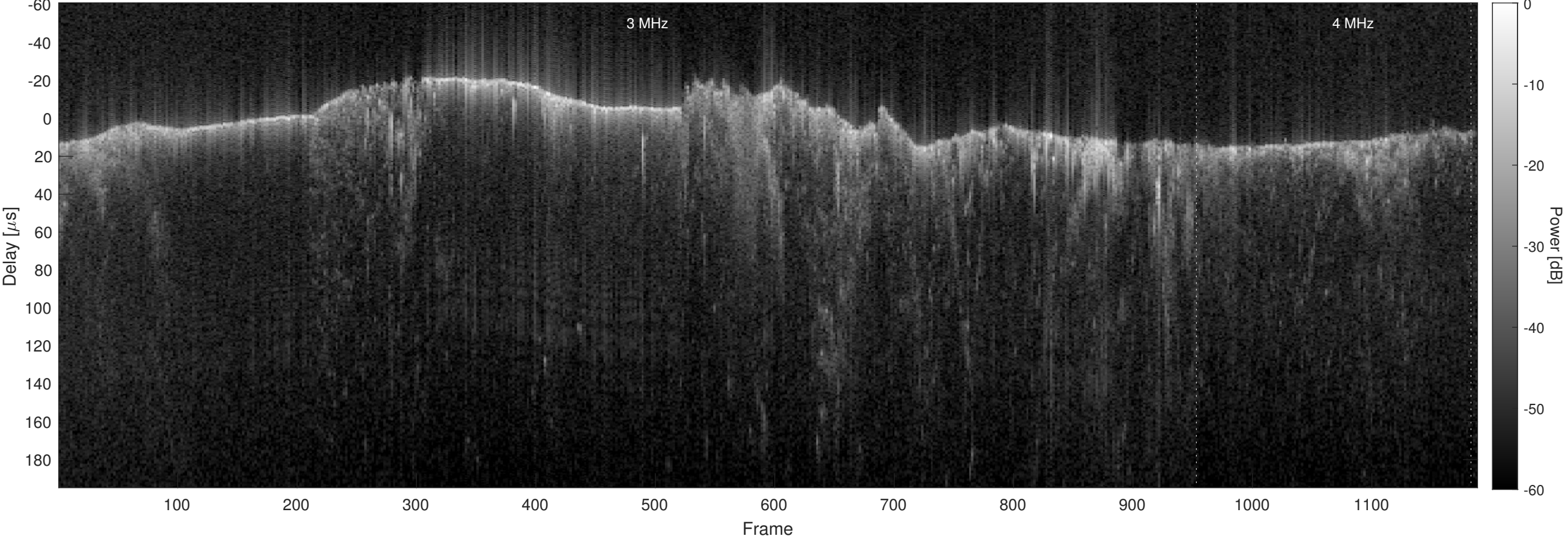
Orbit 4928, Optimized, No Window, Channel 2
