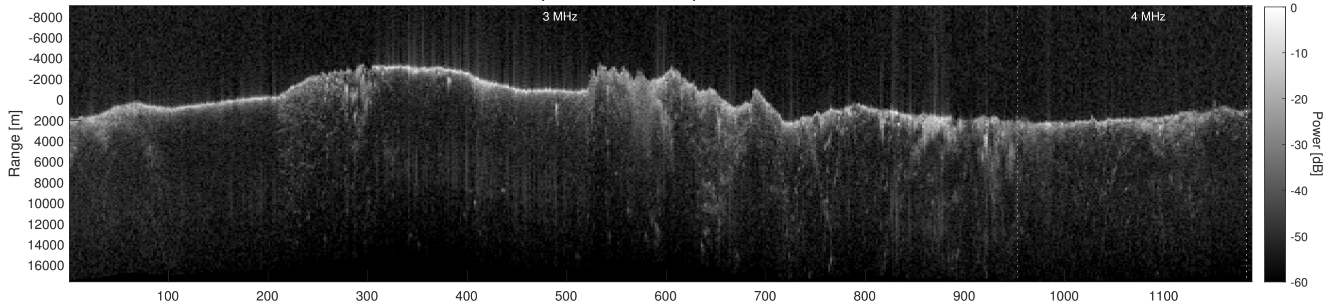
Orbit 4928, Depth-Corrected Cluttergram
