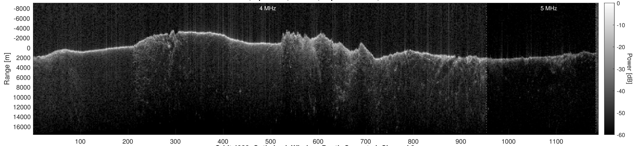
Orbit 4928, Optimized, Window, Depth-Corrected, Channel 2
