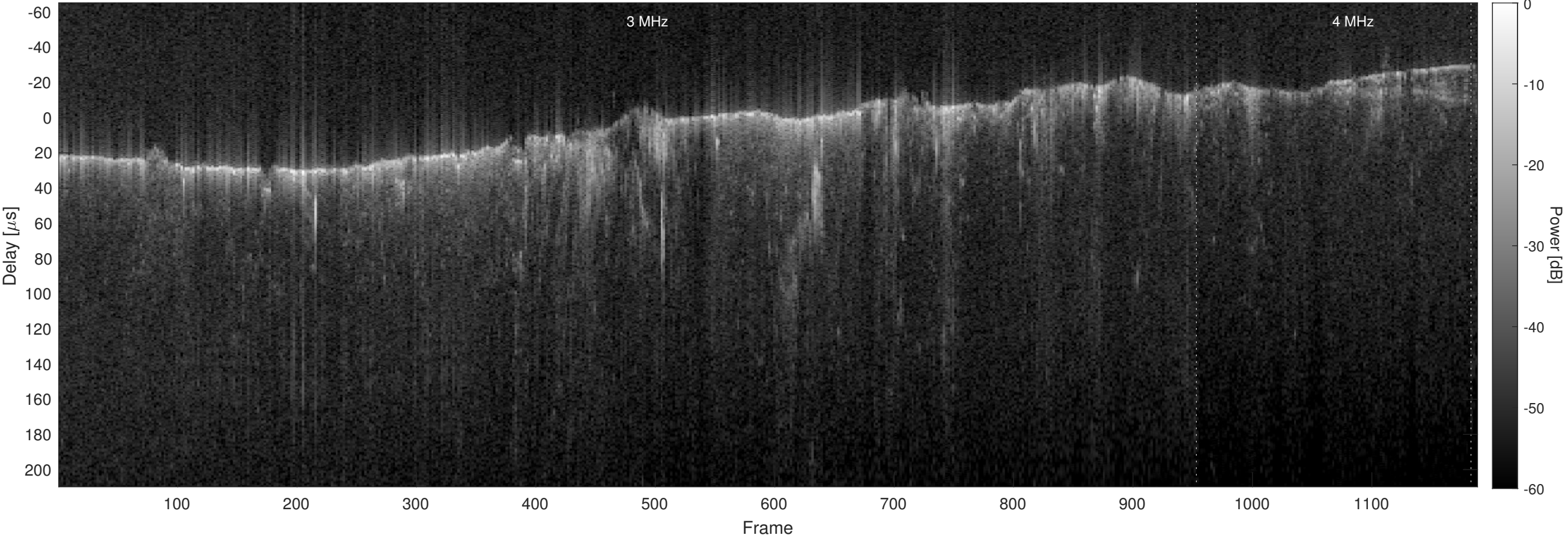
Orbit 4929, Optimized, No Window, Channel 2
