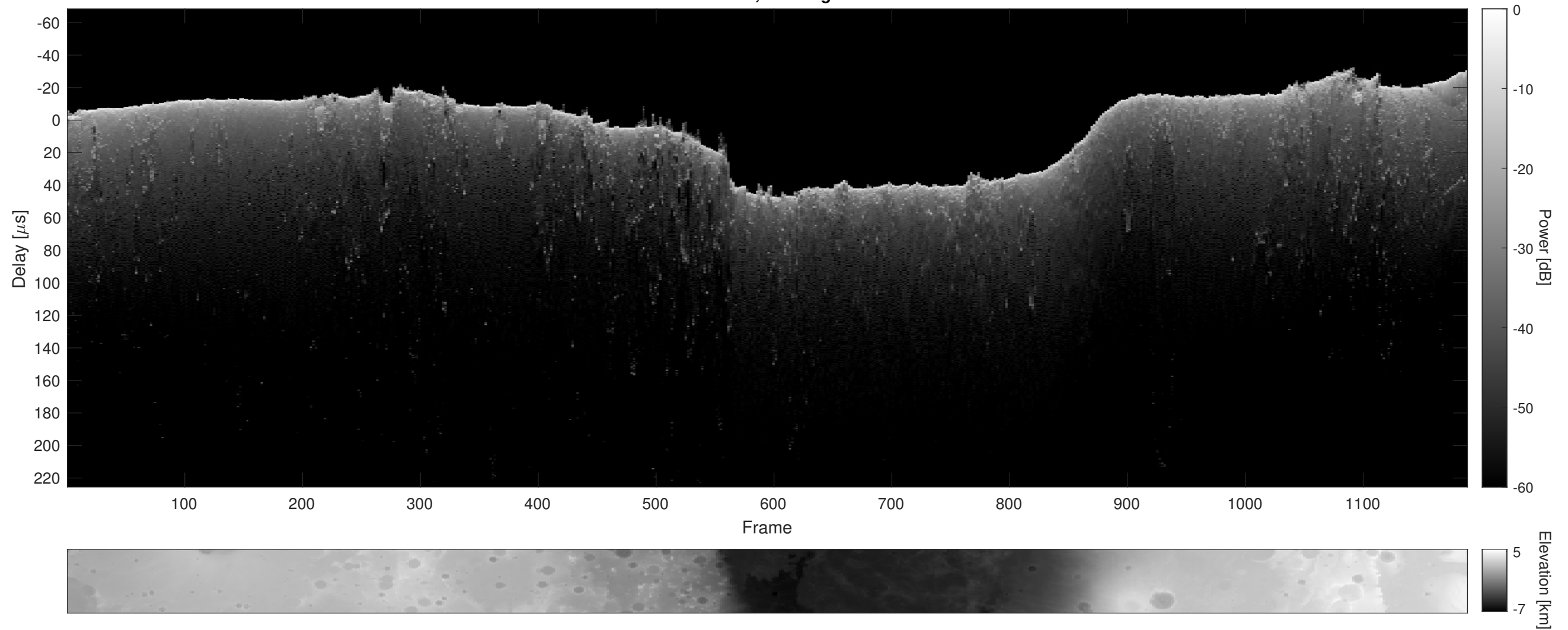
Orbit 4930, Cluttergram
