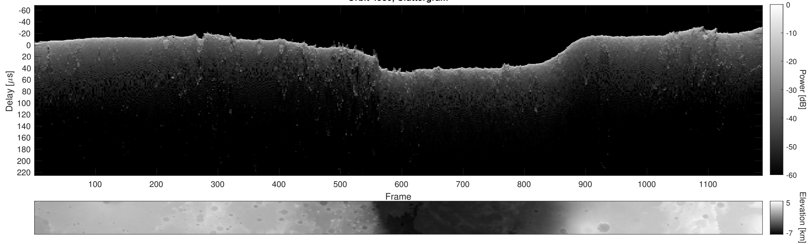
Orbit 4930, Cluttergram
