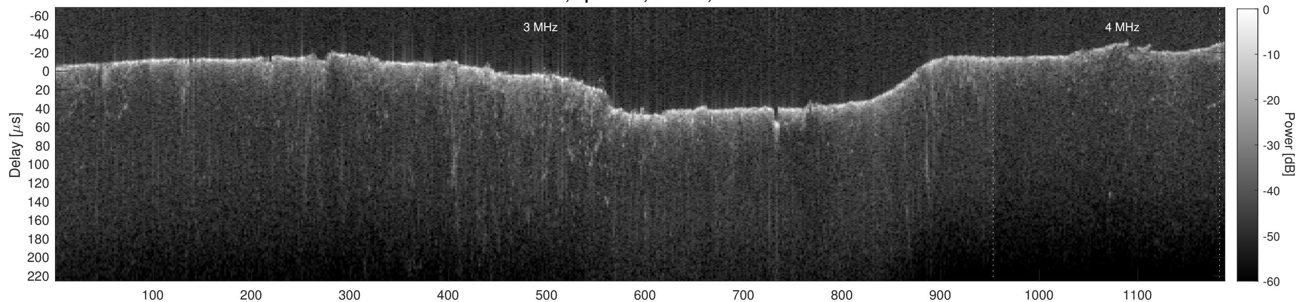
Orbit 4930, Cluttergram
