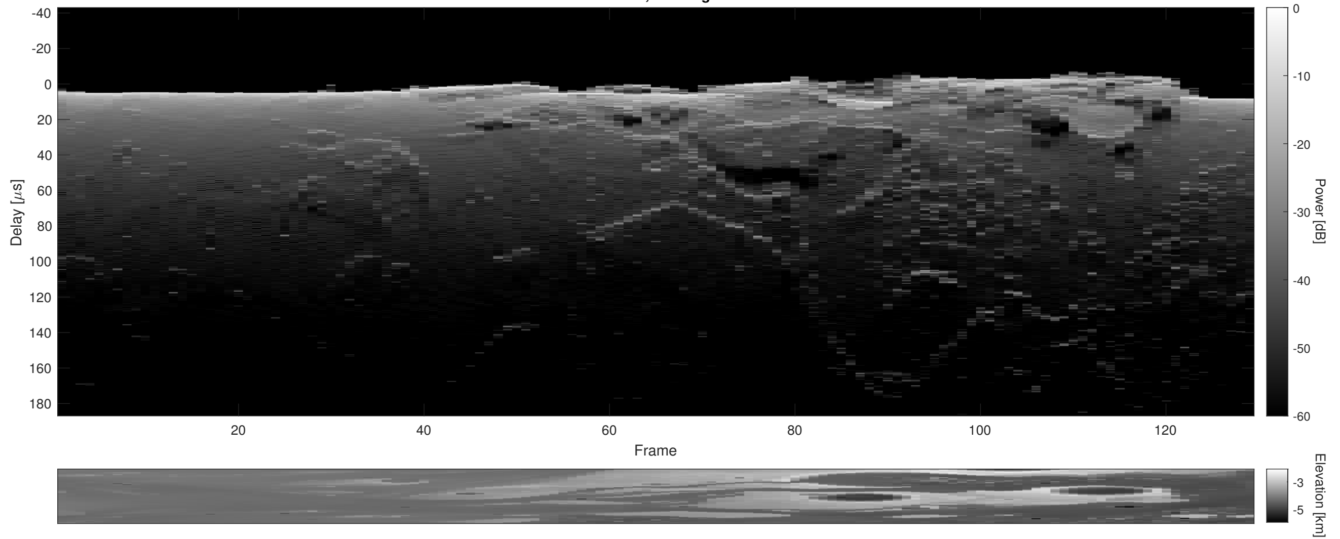
Orbit 4931, Cluttergram
